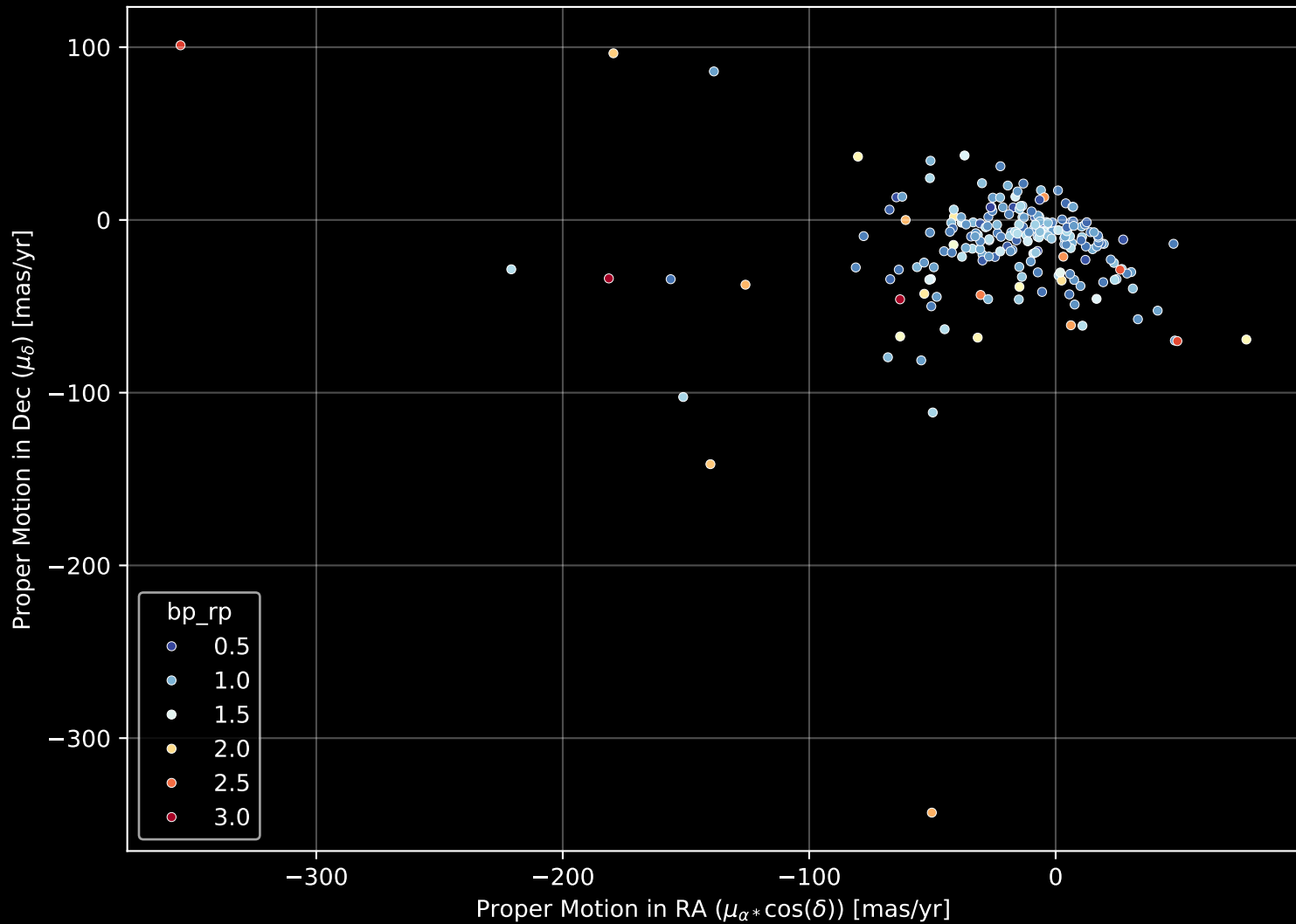
APOGEE DR17 Field: [219+65_MGA] Proper Motion Diagram (n= 212)
