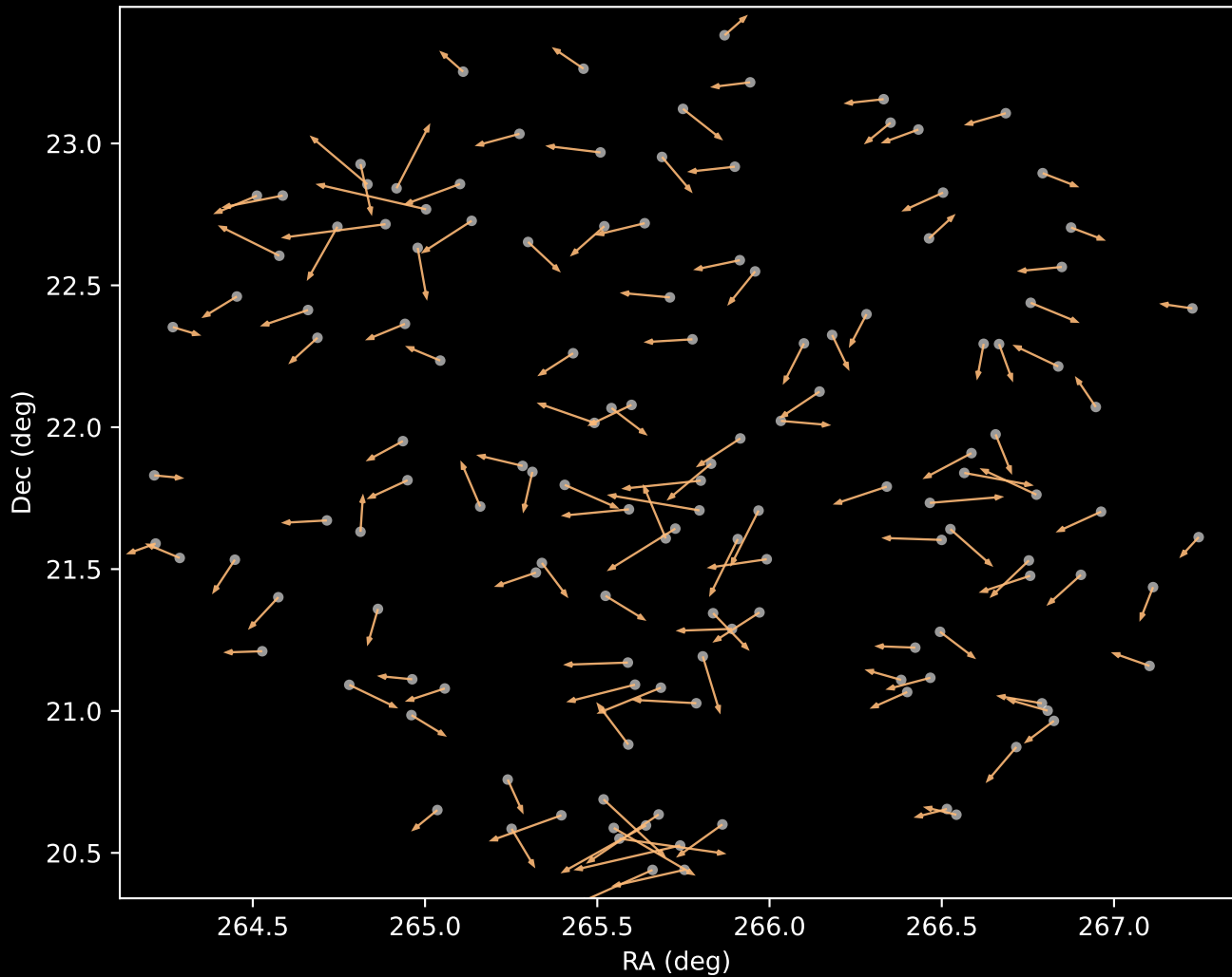
APOGEE DR17 Cluster 3 Proper Motion Vectors (n=138)
